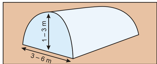
Figure 6: Typical shape and dimensions of a composting windrow.
